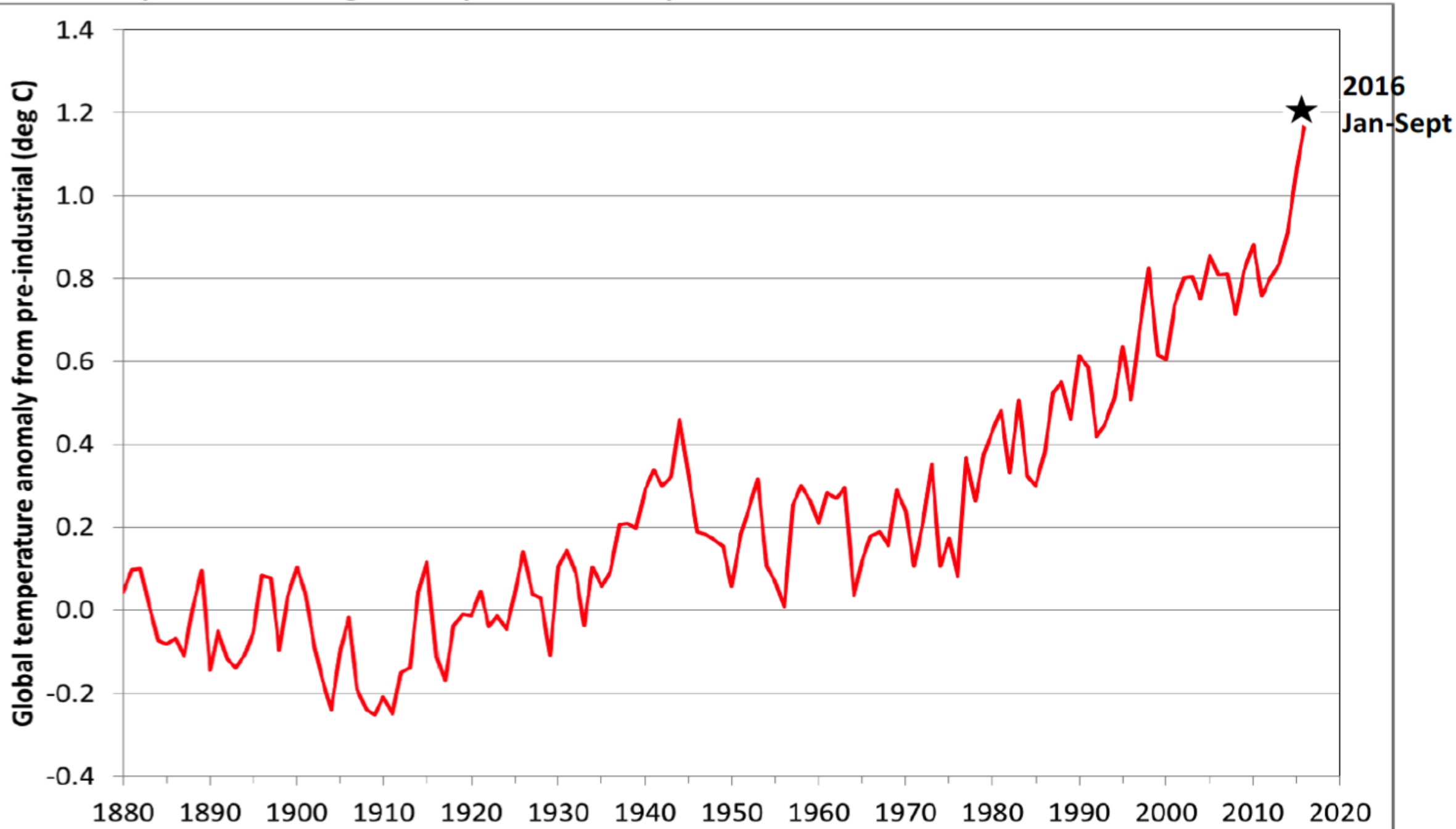
Global Temperature change from pre-industrial period
