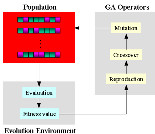
Genetic Algorithm Evolution Flow
