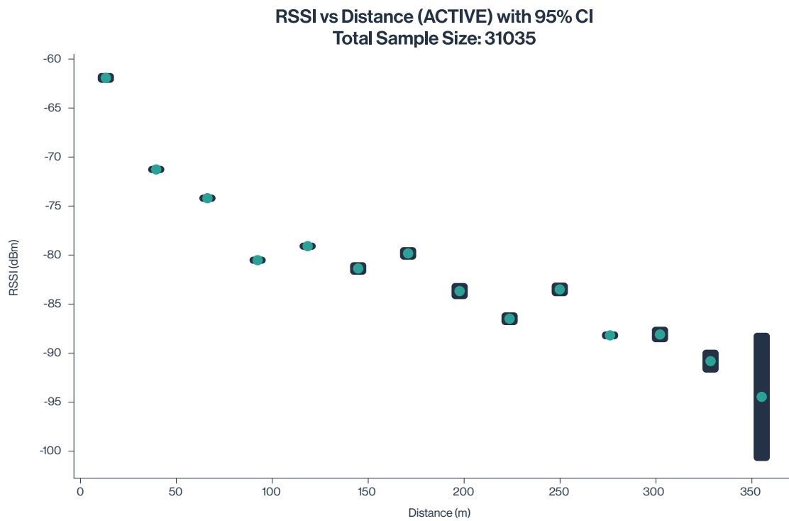
Figure 20. RSSI vs. distance
